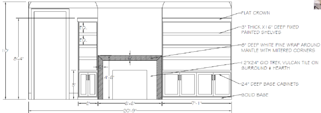
FAMILY ROOM FIREPLACE & BUILT-IN ELEVATION LOT 120 AVENUE DOWNS
