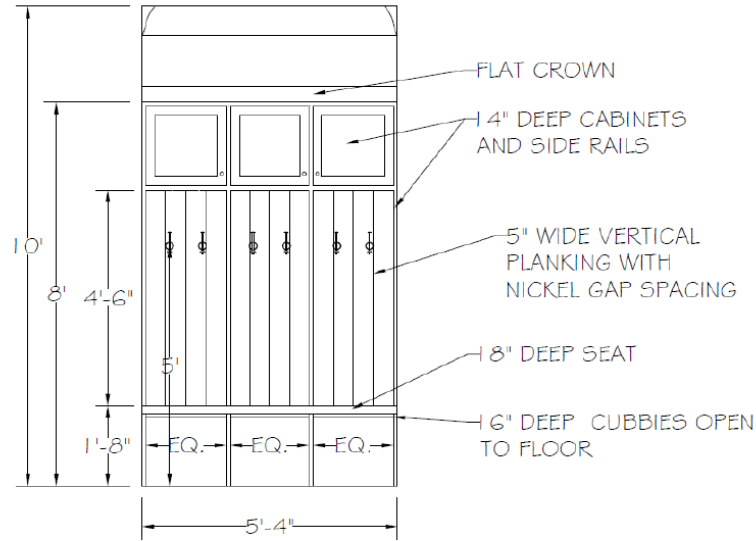
○ MUDROOM BUILT-IN ELEVATION LOT 120 AVENUE DOWNS
