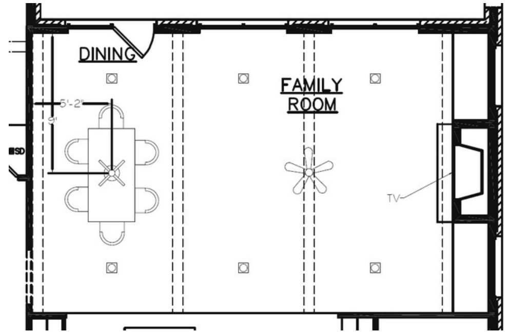
BEAM LAYOUT
